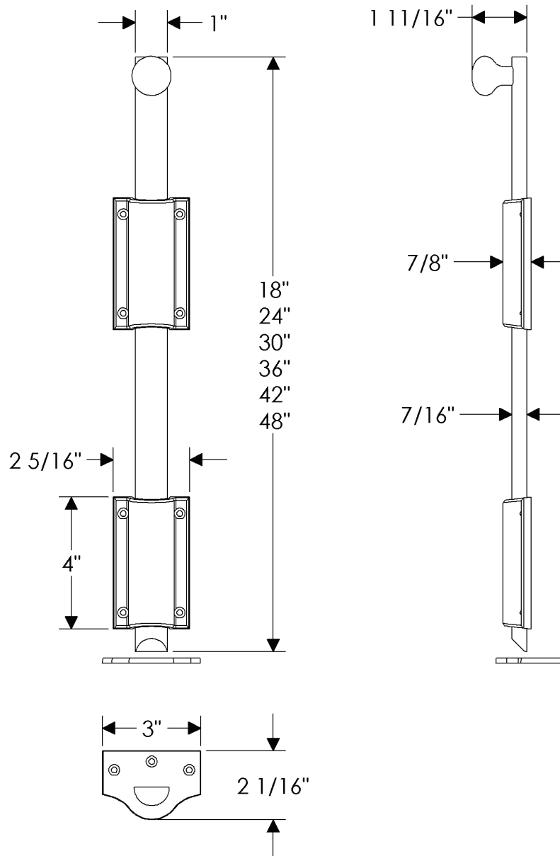
MB12 Surface Bolt Rectangular Mounting Bracket
