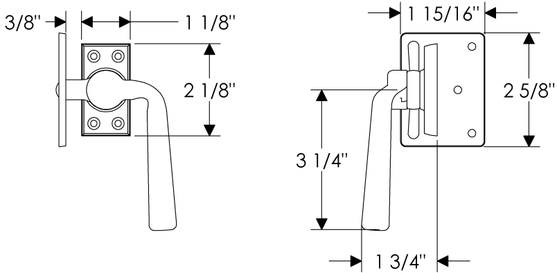
LC300 Casement Latch with LC305 Universal Strike (Left hand shown)
