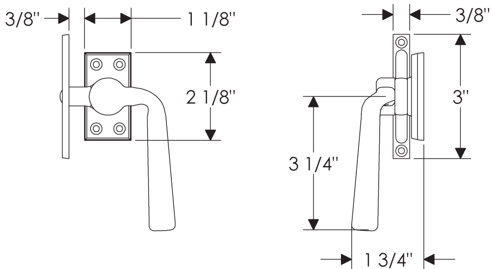
LC300 Casement Latch with LC303 Mortise Strike (Left hand shown)
